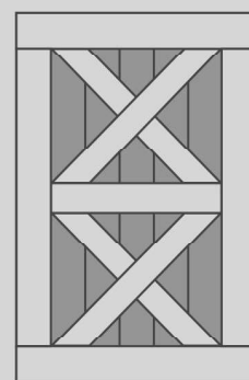
Double X-brace (BD008)
