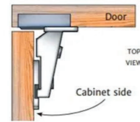
OPTION 1: Full overlay hinge
