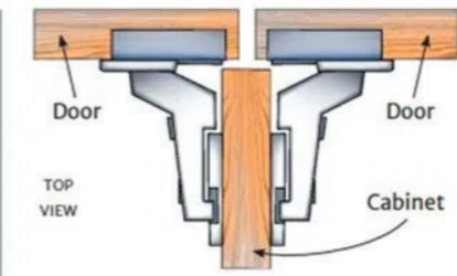
OPTION 2: Half overlay hinge
