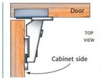
OPTION 4: 165° opening angle hinge
