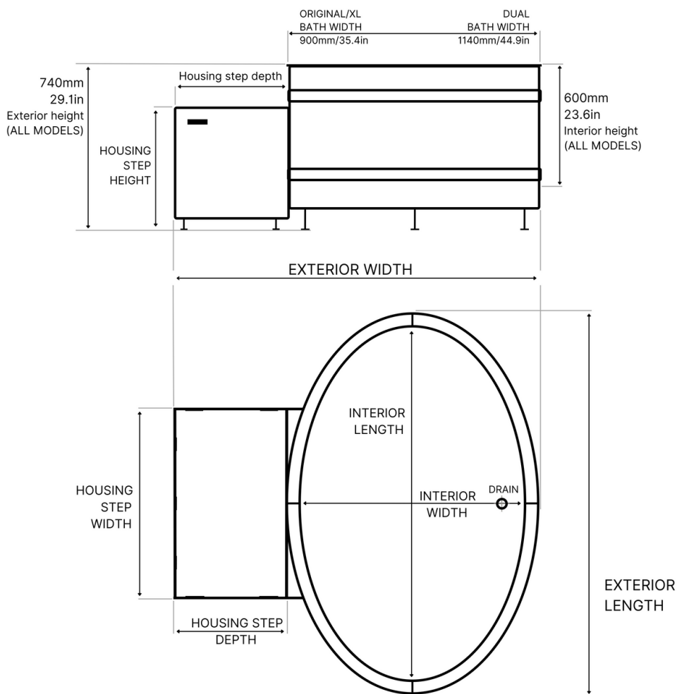
Odin Ice Baths Dimensions Guide (image not to scale)
