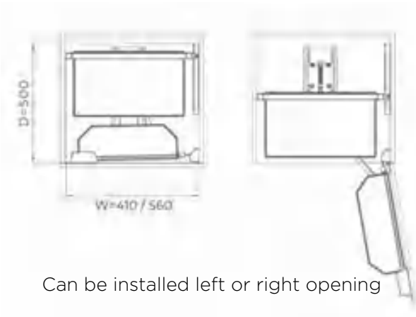
SHEARER PRO OPEN OUT TANDEM PANTRY UNIT - WITH SOFT CLOSE
