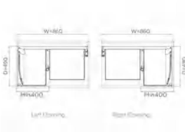
DIAMOND MAGIC CORNER PULL OUT KITCHEN STORAGE - WITH SOFT CLOSE
