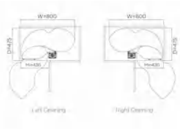
DIAMOND SWING OUT LEMANS KITCHEN CORNER STORAGE - WITH SOFT CLOSE
