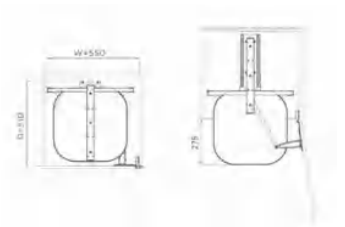
SHEARER TOURBILLON ROTATING PANTRY UNIT - WITH SOFT CLOSE
