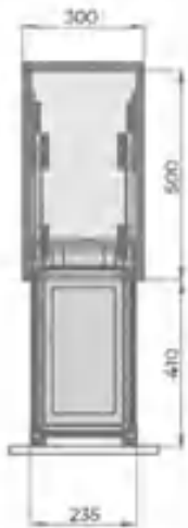
SINGLE SLIDE OUT CONCEALED WASTE BIN - BOTTOM MOUNTED
