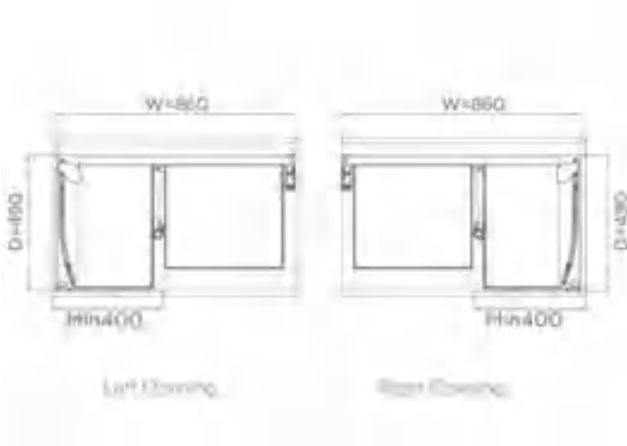
SHEARER PRO MAGIC CORNER PULL OUT KITCHEN STORAGE - WITH SOFT CLOSE
