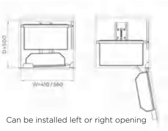
DIAMOND OPEN OUT TANDEM PANTRY UNIT - WITH SOFT CLOSE
