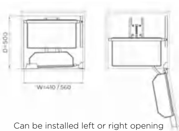
SHEARER OPEN OUT TANDEM PANTRY UNIT - WITH SOFT CLOSE
