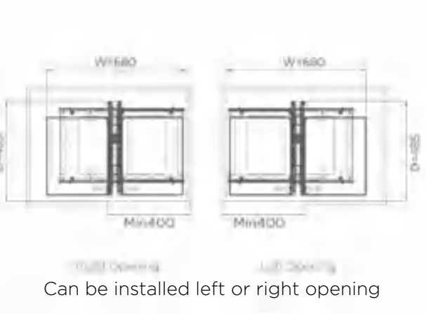
SHEARER PRO SHOW HAND MAGIC CORNER II PULL OUT KITCHEN STORAGE - WITH SOFT CLOSE
