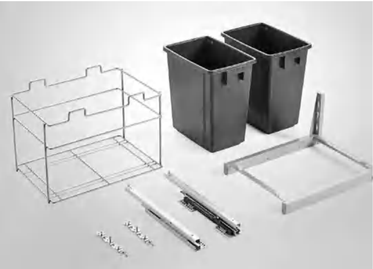
TWIN SLIDE OUT CONCEALED WASTE BIN - BOTTOM MOUNTED
