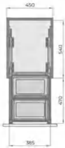
TWIN SLIDE OUT CONCEALED WASTE BIN - BOTTOM MOUNTED
