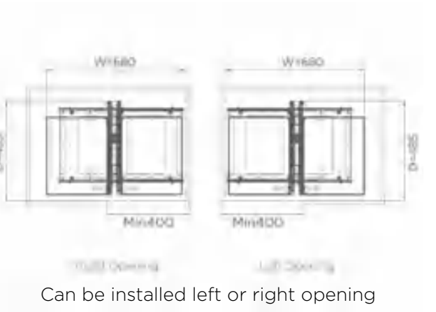
DIAMOND SHOW HAND MAGIC CORNER II PULL OUT KITCHEN STORAGE - WITH SOFT CLOSE
