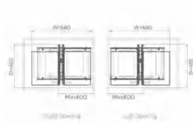
Can be installed left or right opening
