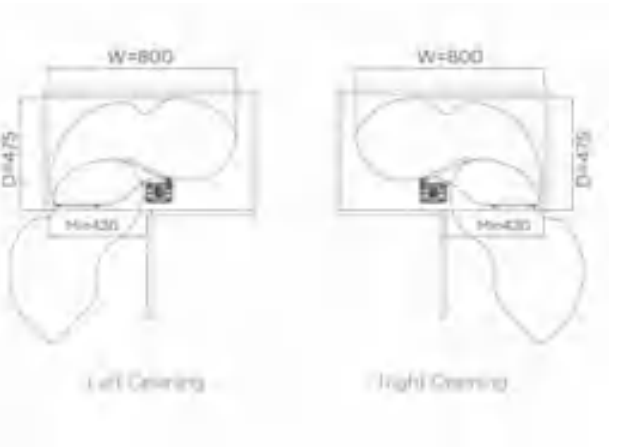
SHEARER SWING OUT LEMANS KITCHEN CORNER STORAGE - WITH SOFT CLOSE
