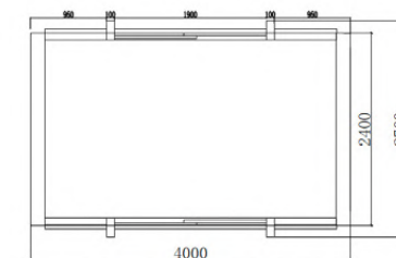
FLOOR PLAN
