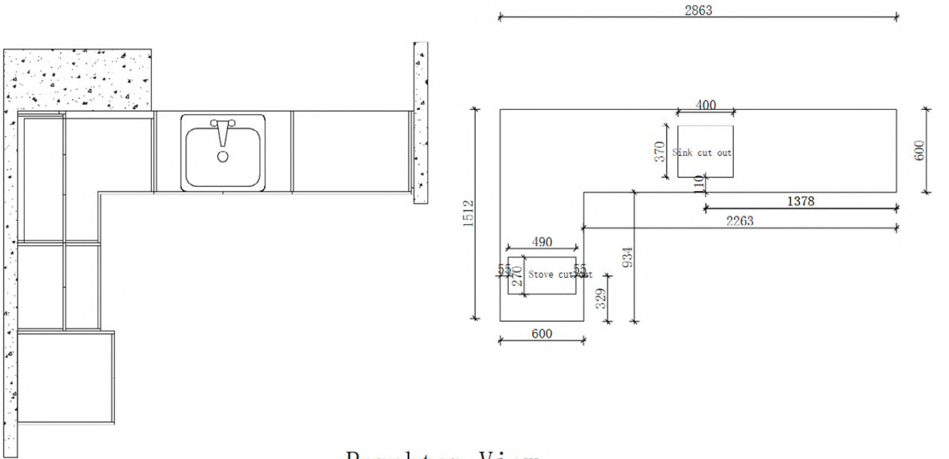
Benchtop View
